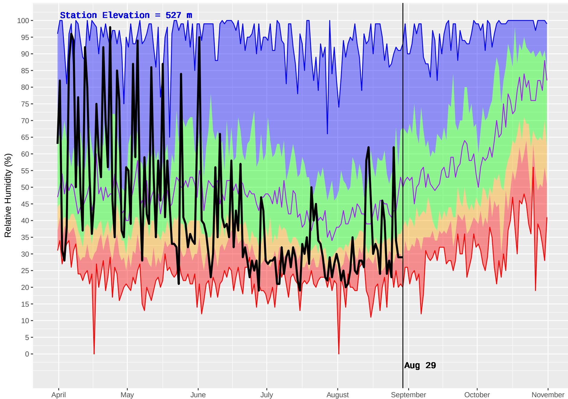
SALMON ARM (346) : Historical (1976–2016) and Current (2017) Noon Relative Humidity
